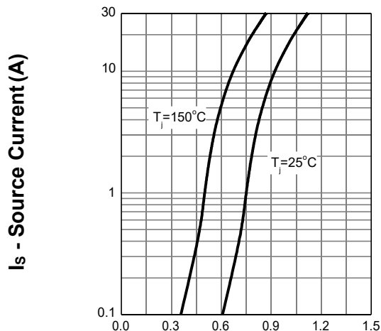
V_{SD} - Source-Drain Voltage (V)
